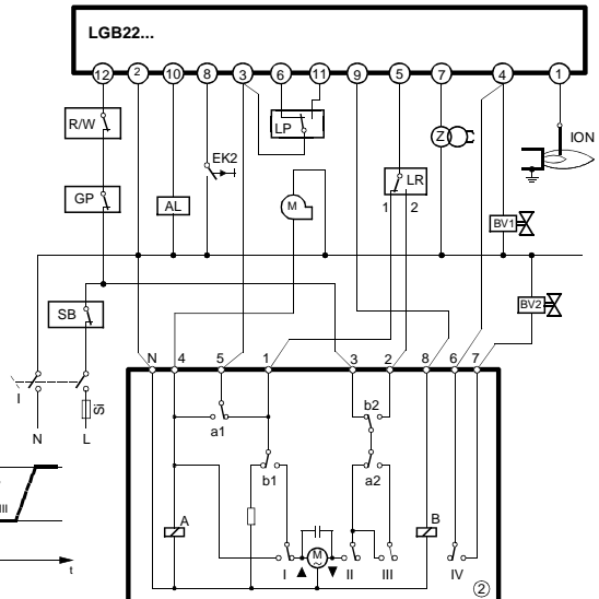
SQN7...424 / 2-stage control 2-wire control
