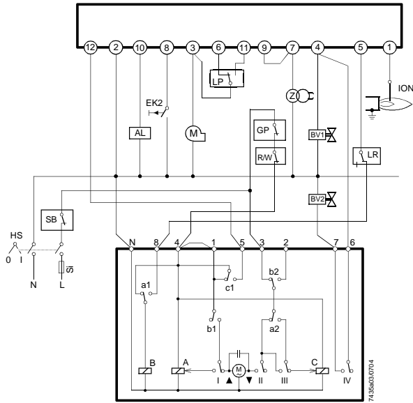
SQN7...244 / 2-stage control
