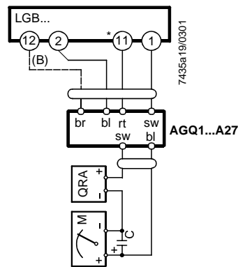
Measuring circuit
