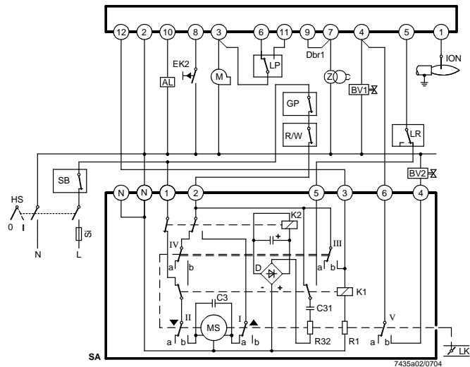
SQN91.140... / 2-stage control
