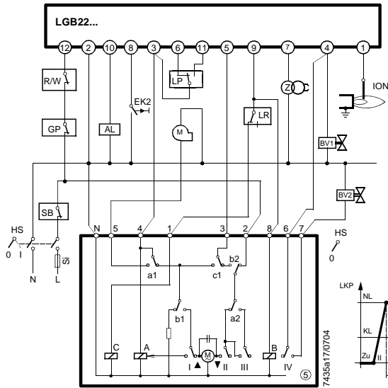
SQN7...454 / 2-stage control Single-wire control
